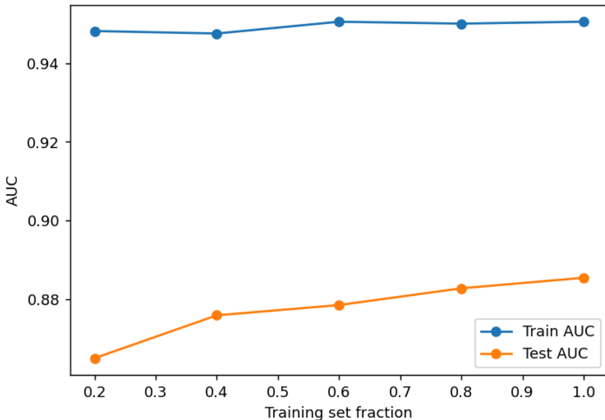
Learning Curve - Tuned Random Forest Pipeline
